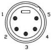
XLR5 Male
