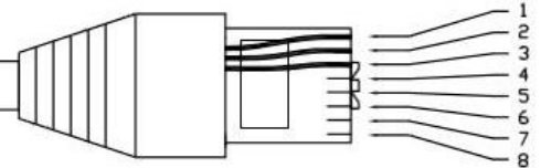
RJ45 8-PIN Male
